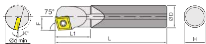
Carbide shank (right shown) 鎢鋼柄 右向示意圖
