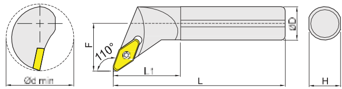
Steel shank (right shown) 鋼柄 右向示意圖
