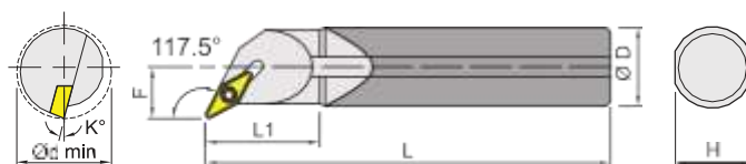
Carbide shank (right shown) 鍍鋼柄 右向示意圖
