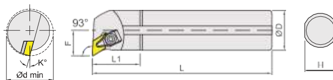
Steel shank (right shown) 鋼柄 右向示意圖
