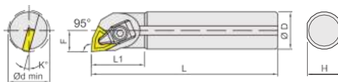
Steel shank (right shown) 鋼柄 右向示意圖
